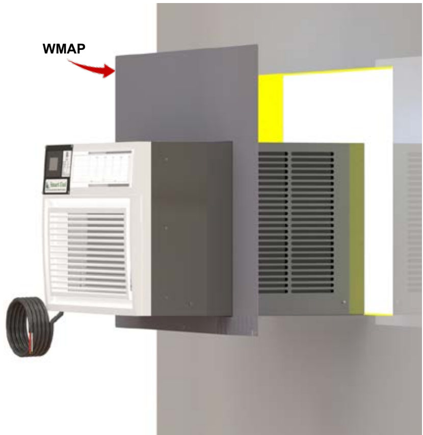
Illustration of Bebco Through-Wall Air Conditioner installation through an oversized wall opening
